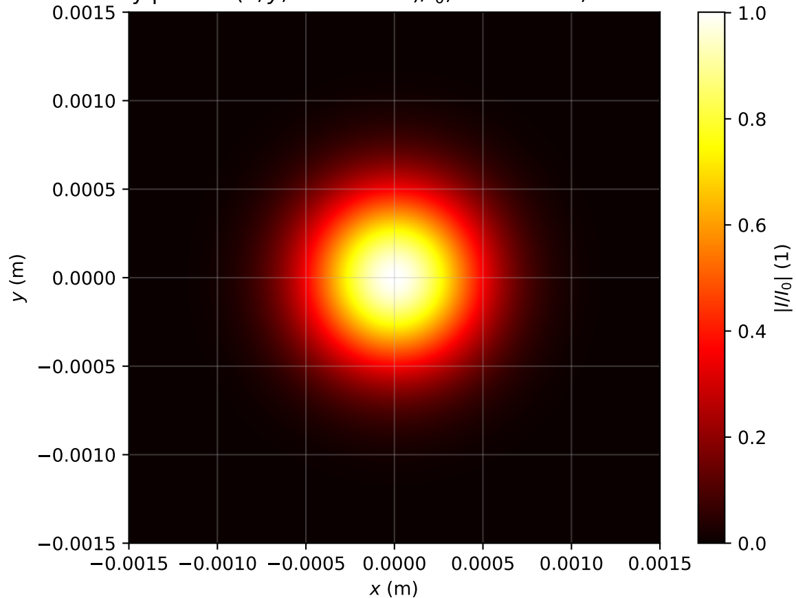
Intensity profile I(x, y, z = 0.159m)/I_0 , Pin=0.3Pcr, artificial time
